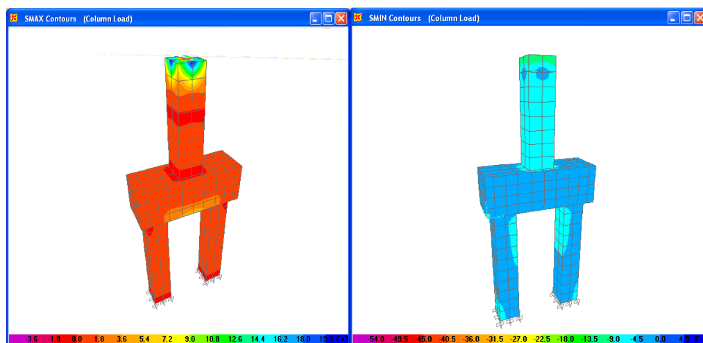
(a) Principal Compressive Stress
