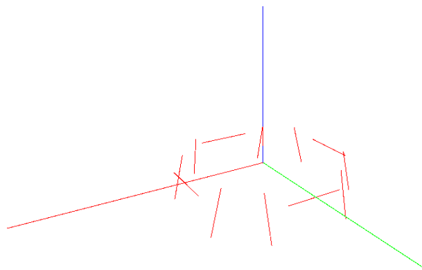
Figure 4.4: Refined Strut and Tie Layout for Four Piles Pile Cap (Span/Depth=2)
