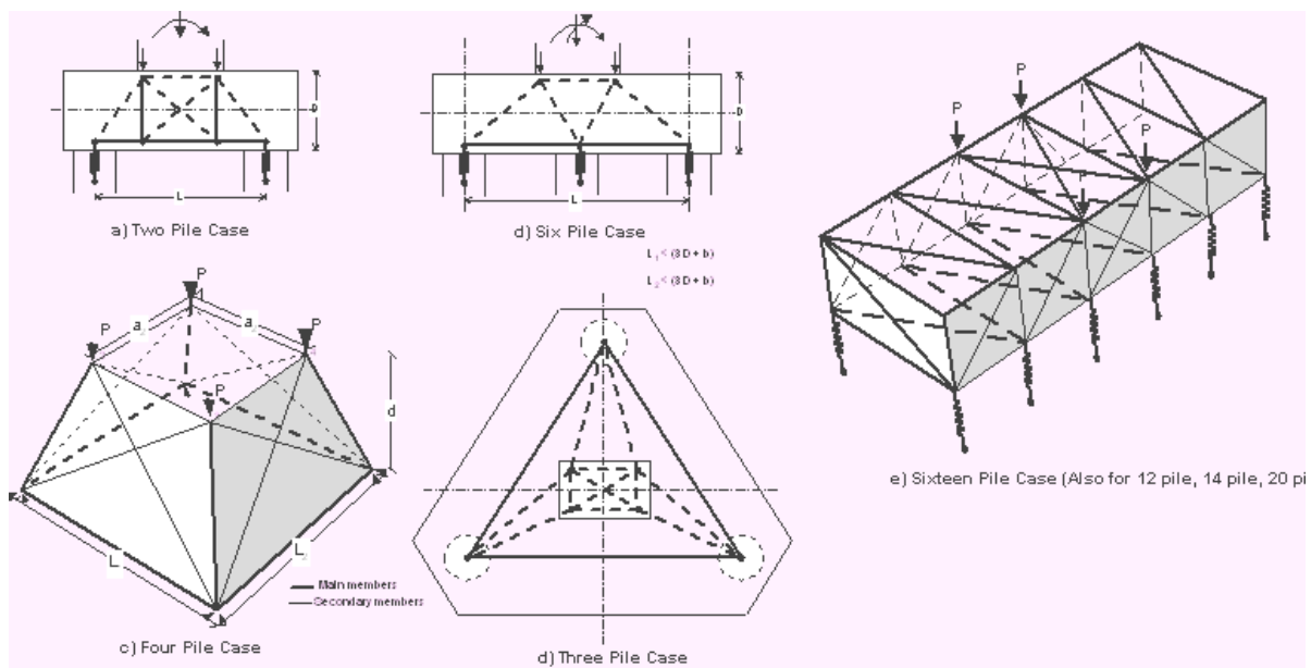
Figure 2.1: Modified 3- D Truss Model for Pile Caps (Nukulchai & Anwar, 1996)
