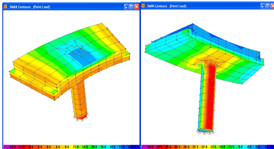
(a)Principal Tensile Stress
