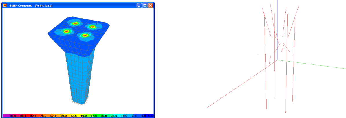
Figure 4.6: Principal Compressive Stress Contours of Pier Head under Point Loading & Extracted Strut and Tie Layout
