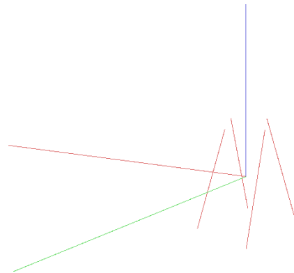
Figure 4.5: Refined Strut and Tie Layout for Four Piles Pile Cap (Span/Depth=1)
